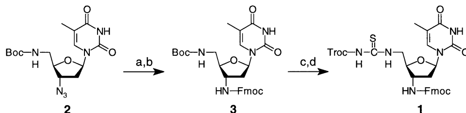
Scheme 1. Synthesis of thymidyl monomer for solid phase synthesis. (a) H_2 , 10% Pd/C, 95% EtOH, 3 h, rt, 99%; (b) 1.1 equiv Fmoc-Cl, 1:1 Dioxane:10% Na_2CO_3 , 30 min, rt, 83%; (c) 30% TFA/DCM, 5 min, rt, 100%; (d) TrocNCS ( 4 ), TEA (2 equiv), DCM, 30 min, rt, 85%.
