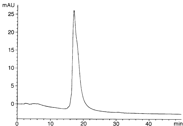
Figure 1. HPLC chromatogram of purified DNG oligomer 7 . Conditions: Alltech macrosphere 300SCX cation exchange column. Buffer a: 50 mM TRIS buffer, pH 6.4; Buffer b: 2 M guanidinium hydrochloride, 50 mM TRIS buffer, pH 6.4. 0 to 100% gradient of b over 45 min. at 1.3 mL/min. HP 1090 HPLC equipped with UV detector, \lambda = 260 \text{ nm} . Retention time = 17.1 min.
