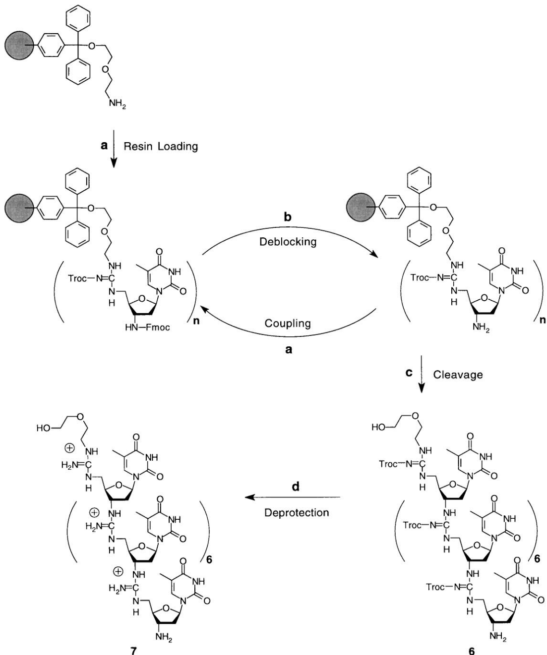
Scheme 3. Solid-phase synthesis of DNG. (a) Coupling: monomer (1), HgCl 2 (2 equiv), TEA (2 equiv); (b) Deblocking: 20% piperidine in DMF; (c) Cleavage: 3% dichloroacetic acid in DCM; (d) Deprotection: acetic acid/zinc powder.
